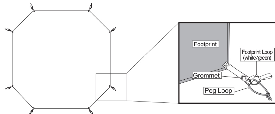
Moonlight tent 4 Footprint
